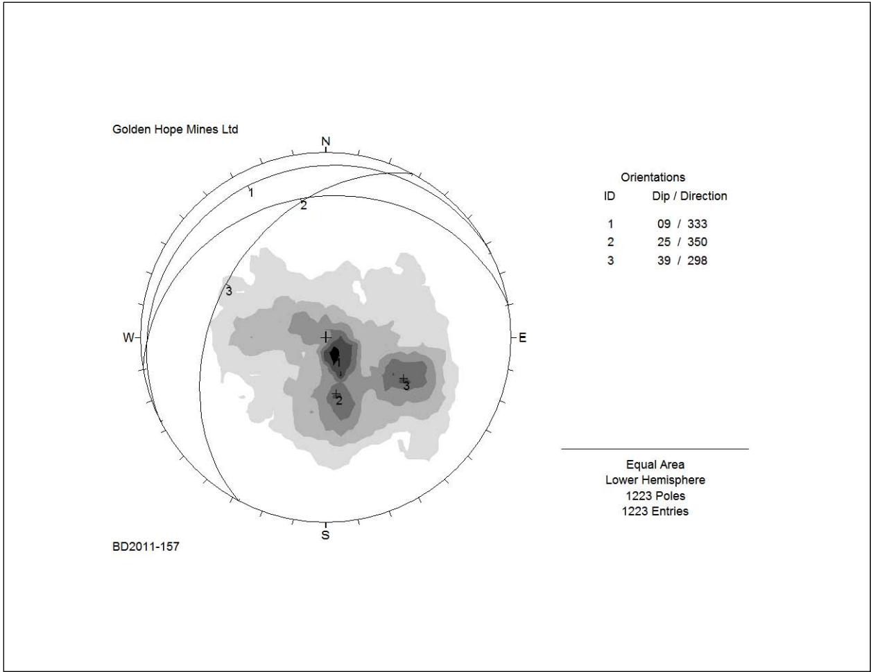
Figure 1. BD2011-157 -- Stereonet showing a cluster of relatively flat lying structures. Stereonet montrant un groupe de structures sub-horizontale.
